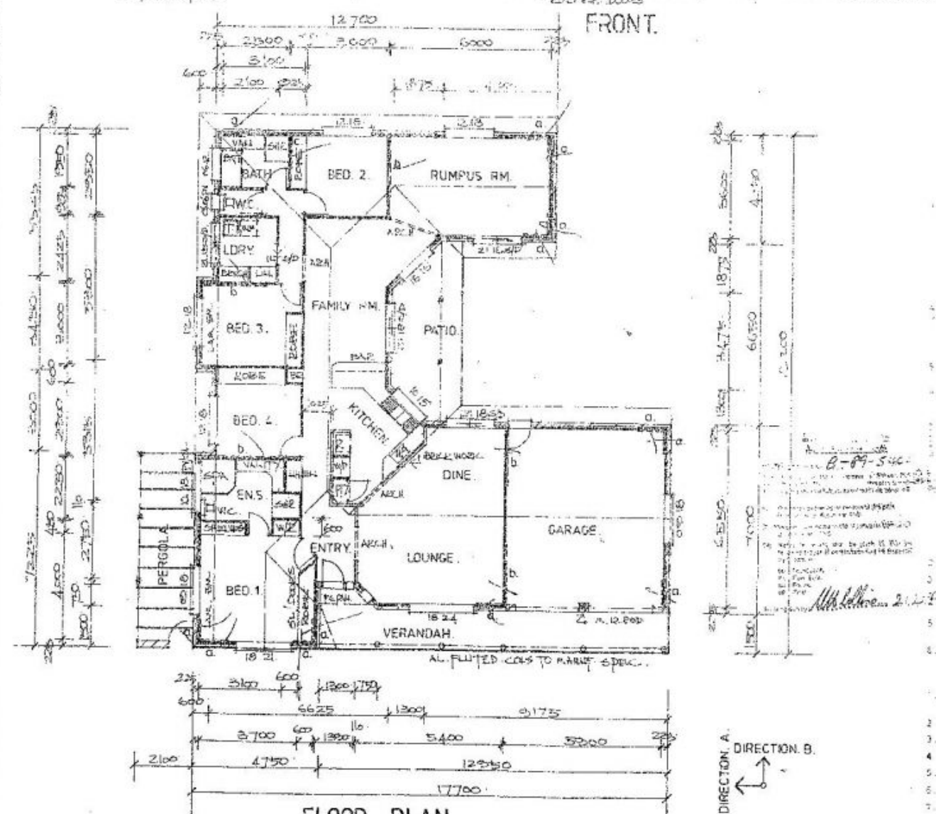
FLOOR PLAN.
