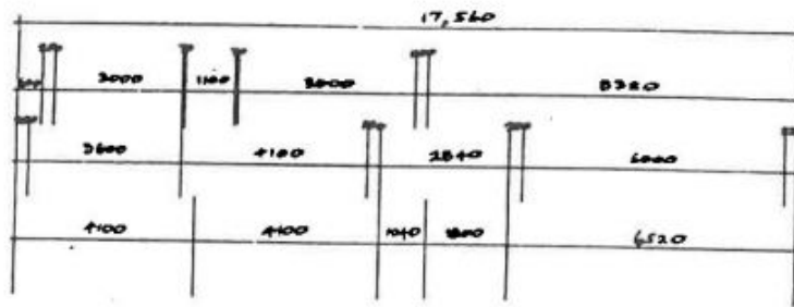
Rear Elevation.
