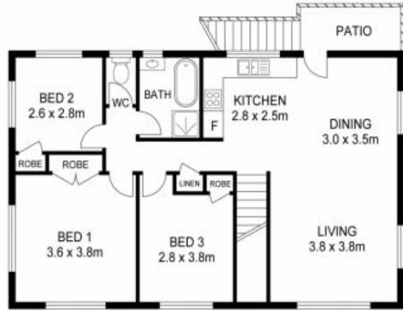
UPPER LEVEL
